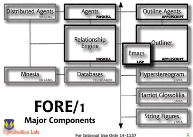
FORE/1 Architecture
