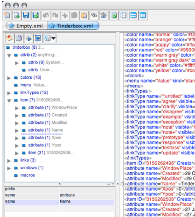
Tinderbox Data in EditiX
