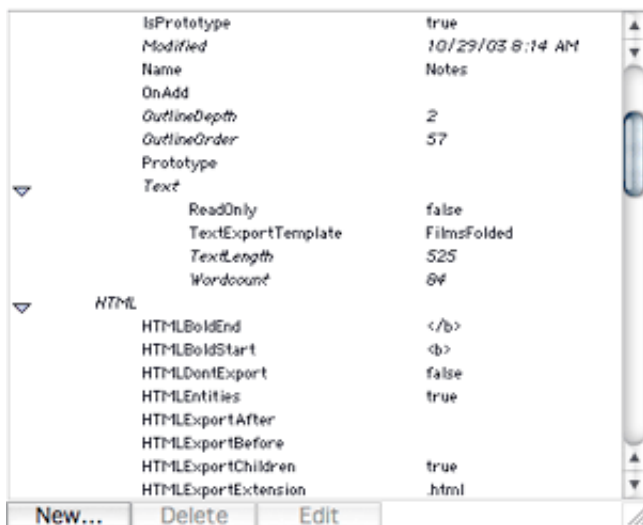
The Get Info Window
