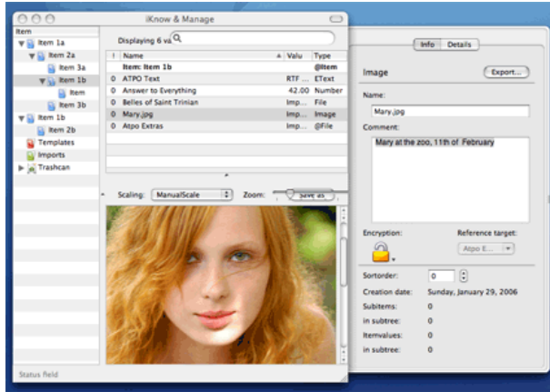
iKnow Info Panel and Value Alias
