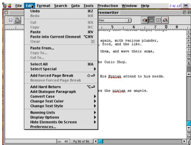
Edit Menu
