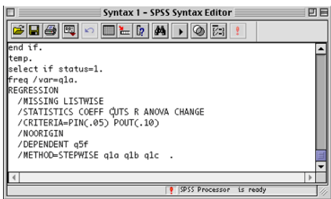
Syntax Regression
