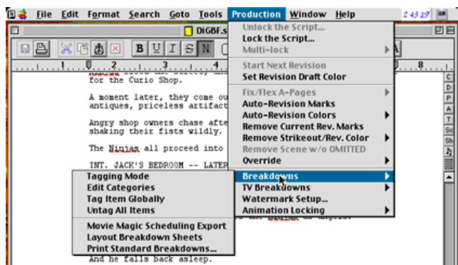
Advanced Features
