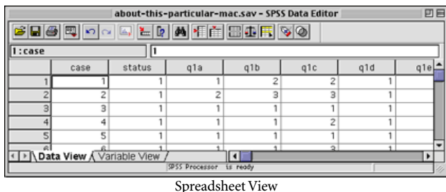
Spreadsheet View
